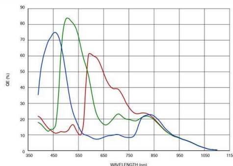
MV-CU050-30GC 响应曲线
